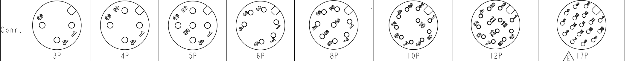
Pin Assignments Front View
