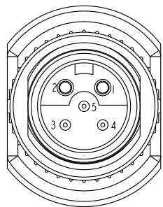
Pin Assignments Front View
