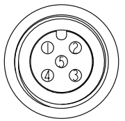
Conn. 2 Pin Assignment Front View
